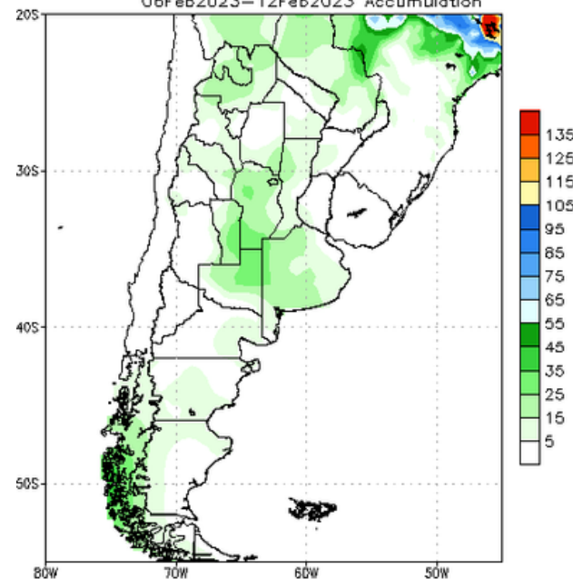
NCEP GFS Ensemble Forecast 8–14 Day Precipitation (mm) from: 30Jan2023 06Feb2023–12Feb2023 Accumulation
