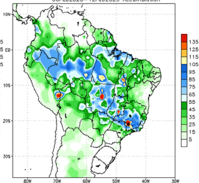
NCEP GFS Ensemble Forecast 8–14 Day Precipitation (mm) from: 30Jan2023 06Feb2023–12Feb2023 Accumulation
