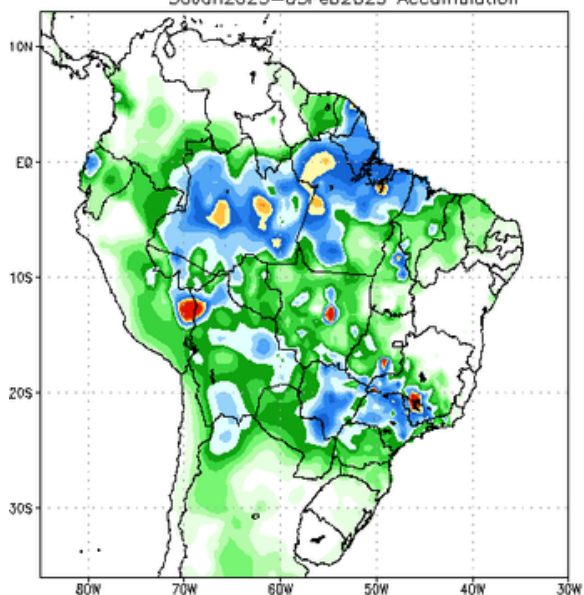
NCEP GFS Ensemble Forecast 1–7 Day Precipitation (mm) from: 30Jan2023 30Jan2023–05Feb2023 Accumulation
