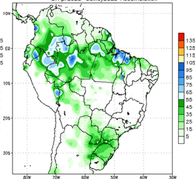
NCEP GFS Ensemble Forecast 8–14 Day Precipitation (mm) from: 20Apr2023 27Apr2023–03May2023 Accumulation
