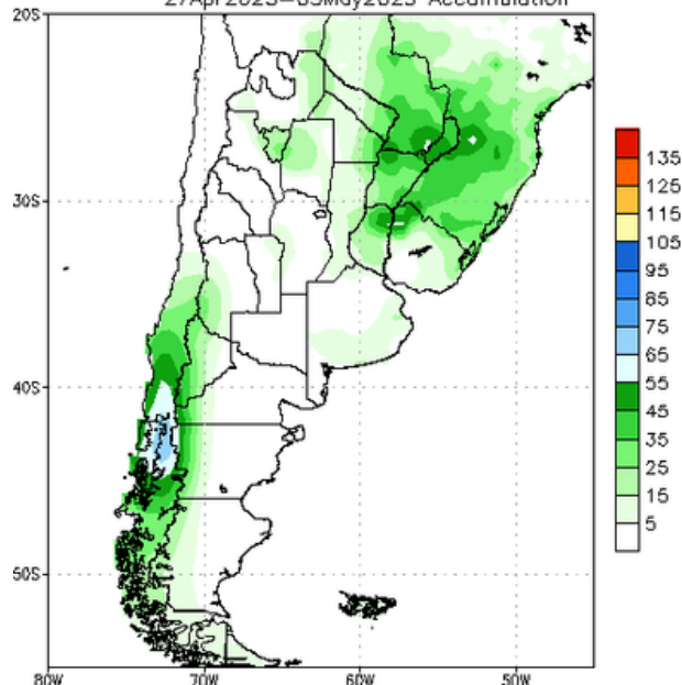
NCEP GFS Ensemble Forecast 8–14 Day Precipitation (mm) from: 20Apr2023 27Apr2023–03May2023 Accumulation
