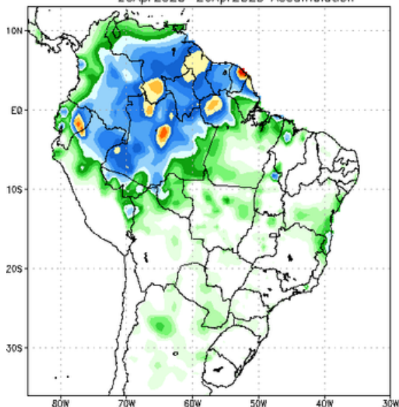
NCEP GFS Ensemble Forecast 1–7 Day Precipitation (mm) from: 20Apr2023 20Apr2023–26Apr2023 Accumulation
