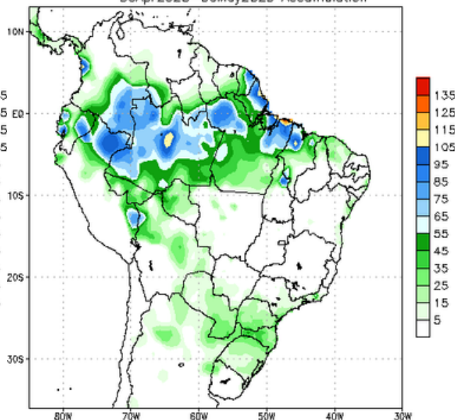
NCEP GFS Ensemble Forecast 8–14 Day Precipitation (mm) from: 23Apr2023 30Apr2023–06May2023 Accumulation
