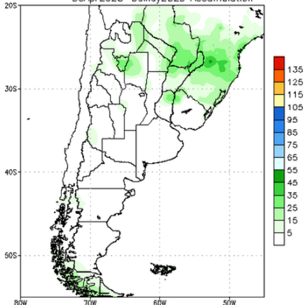
NCEP GFS Ensemble Forecast 8–14 Day Precipitation (mm) from: 23Apr2023 30Apr2023–06May2023 Accumulation
