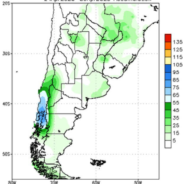
NCEP GFS Ensemble Forecast 1–7 Day Precipitation (mm) from: 24Apr2023 24Apr2023–30Apr2023 Accumulation
