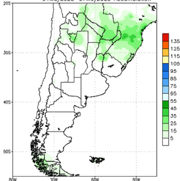
NCEP GFS Ensemble Forecast 8–14 Day Precipitation (mm) from: 24Apr2023 01May2023–07May2023 Accumulation
