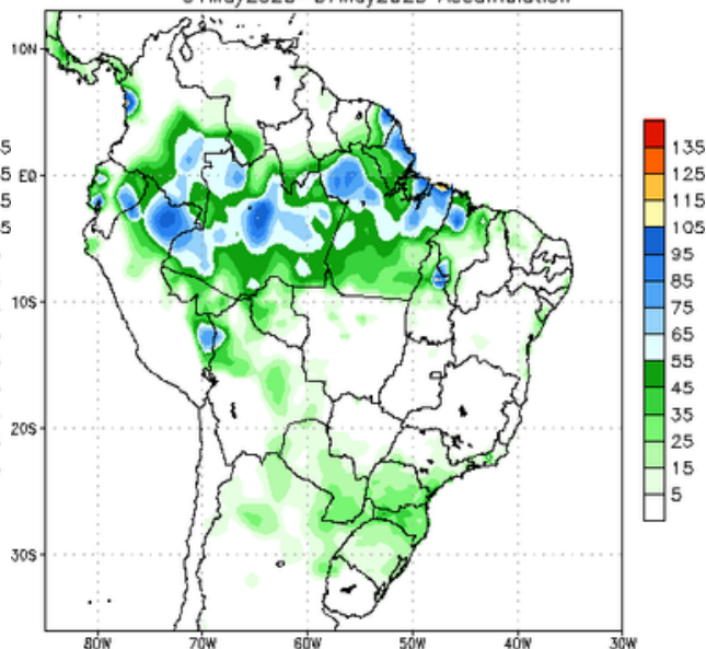
NCEP GFS Ensemble Forecast 8–14 Day Precipitation (mm) from: 24Apr2023 01May2023–07May2023 Accumulation
