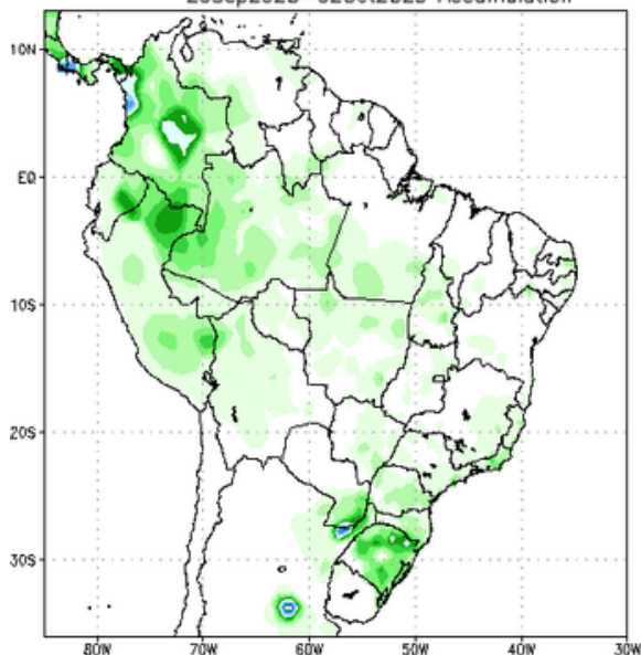
NCEP GFS Ensemble Forecast 1–7 Day Precipitation (mm) from: 26Sep2023 26Sep2023–02Oct2023 Accumulation
