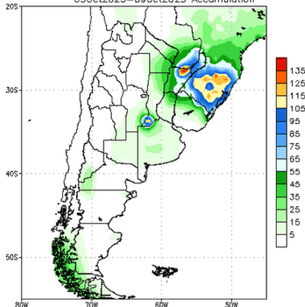
NCEP GFS Ensemble Forecast 8–14 Day Precipitation (mm) from: 26Sep2023 03Oct2023–09Oct2023 Accumulation
