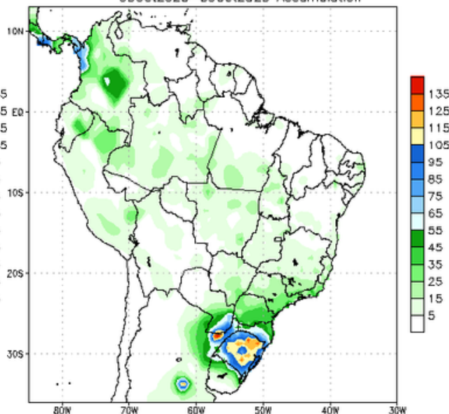
NCEP GFS Ensemble Forecast 8–14 Day Precipitation (mm) from: 26Sep2023 03Oct2023–09Oct2023 Accumulation
