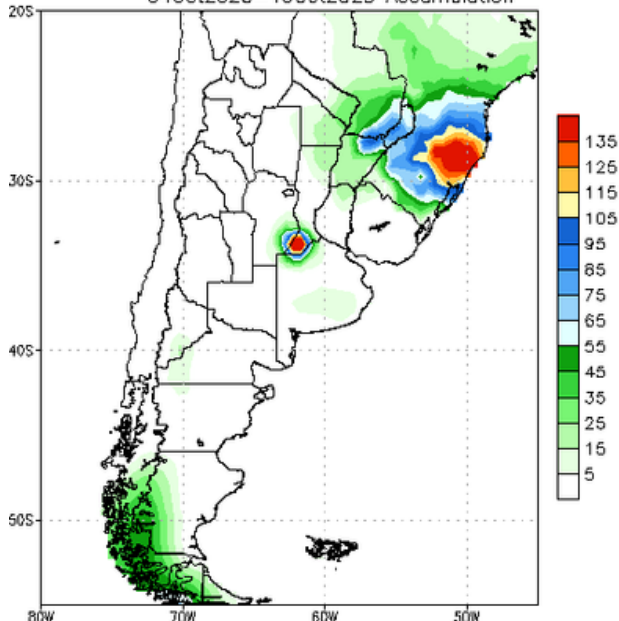
NCEP GFS Ensemble Forecast 1–7 Day Precipitation (mm) from: 04Oct2023 04Oct2023–10Oct2023 Accumulation
