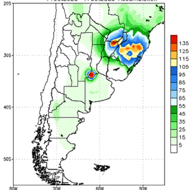
NCEP GFS Ensemble Forecast 8–14 Day Precipitation (mm) from: 04Oct2023 11Oct2023–17Oct2023 Accumulation
