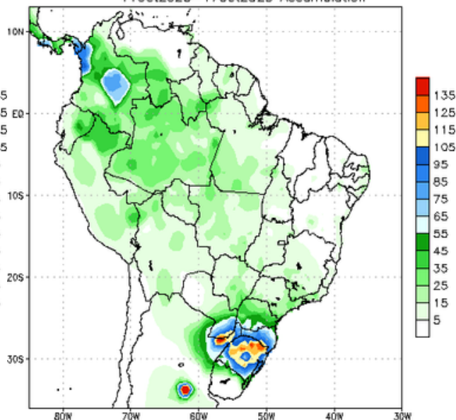
NCEP GFS Ensemble Forecast 8–14 Day Precipitation (mm) from: 04Oct2023 11Oct2023–17Oct2023 Accumulation
