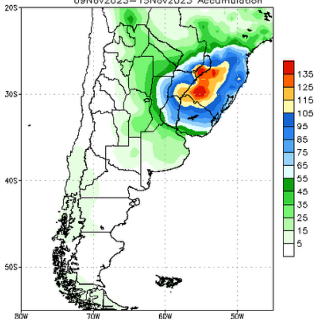
Bias correction based on last 30-day forecast error NCEP GFS Ensemble Forecast 8–14 Day Precipitation (mm) from: 02Nov2023 09Nov2023–15Nov2023 Accumulation
