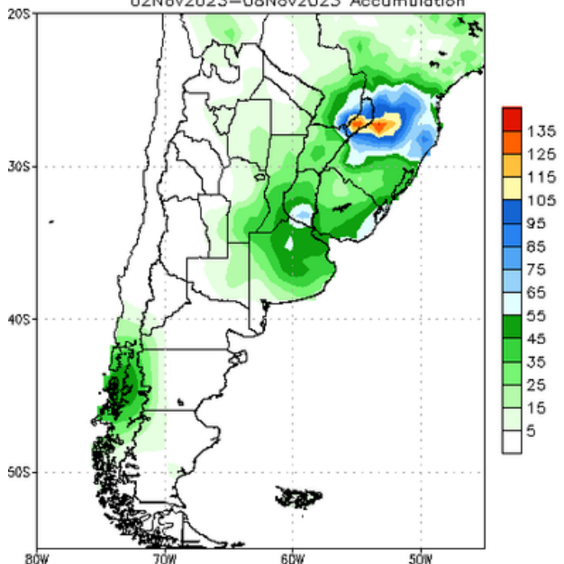
Bias correction based on last 30-day forecast error NCEP GFS Ensemble Forecast 1–7 Day Precipitation (mm) from: 02Nov2023 02Nov2023–08Nov2023 Accumulation
