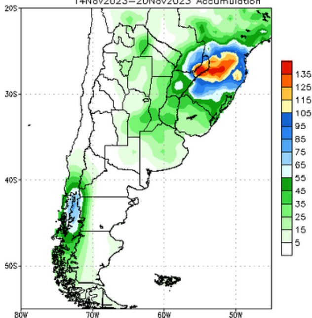
NCEP GFS Ensemble Forecast 8–14 Day Precipitation (mm) from: 07Nov2023 14Nov2023–20Nov2023 Accumulation
