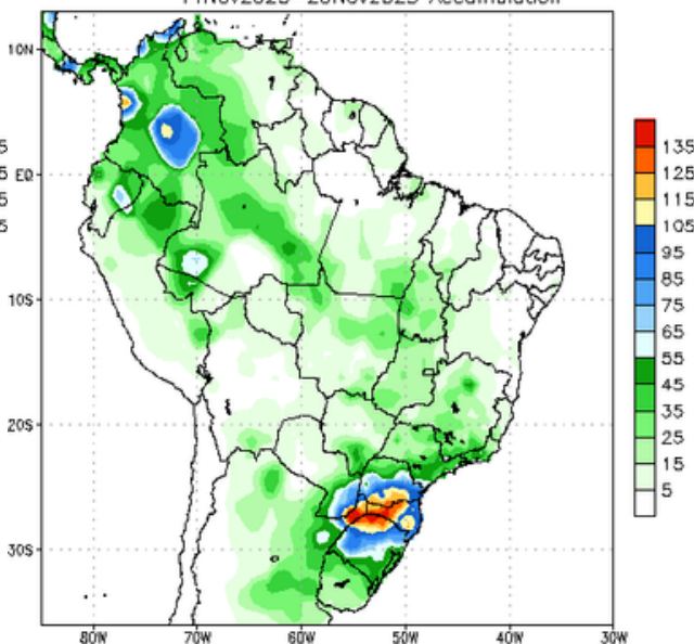
NCEP GFS Ensemble Forecast 8–14 Day Precipitation (mm) from: 07Nov2023 14Nov2023–20Nov2023 Accumulation
