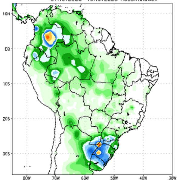
NCEP GFS Ensemble Forecast 1–7 Day Precipitation (mm) from: 07Nov2023 07Nov2023–13Nov2023 Accumulation
