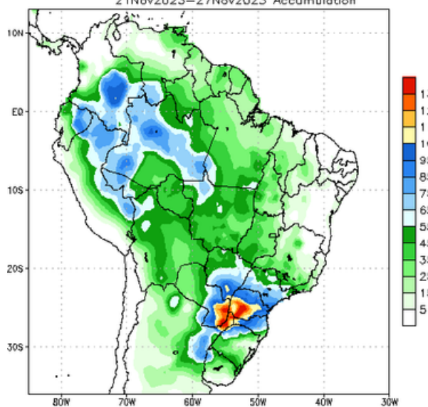
NCEP GFS Ensemble Forecast 1–7 Day Precipitation (mm) from: 21Nov2023 21Nov2023–27Nov2023 Accumulation
