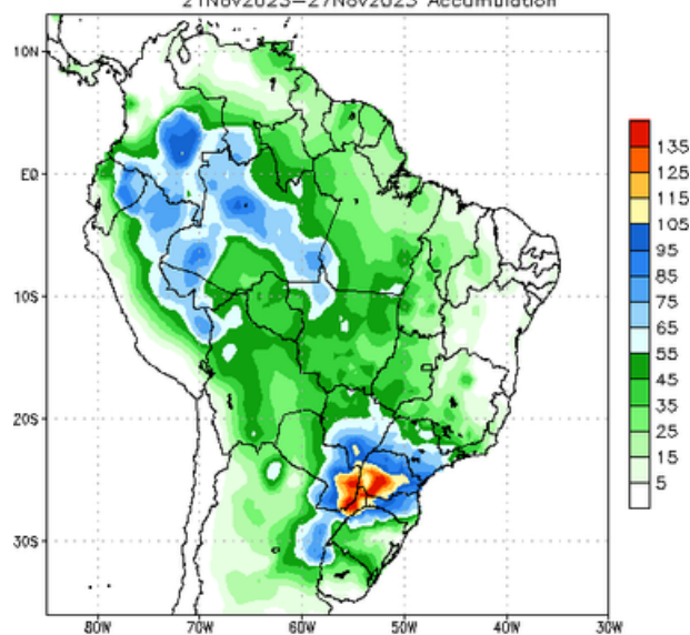
NCEP GFS Ensemble Forecast 1–7 Day Precipitation (mm) from: 21Nov2023 21Nov2023–27Nov2023 Accumulation
