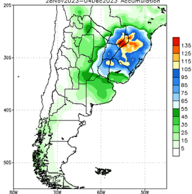
NCEP GFS Ensemble Forecast 8–14 Day Precipitation (mm) from: 21Nov2023 28Nov2023–04Dec2023 Accumulation
