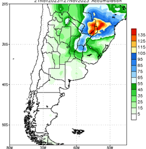
NCEP GFS Ensemble Forecast 1–7 Day Precipitation (mm) from: 21Nov2023 21Nov2023–27Nov2023 Accumulation
